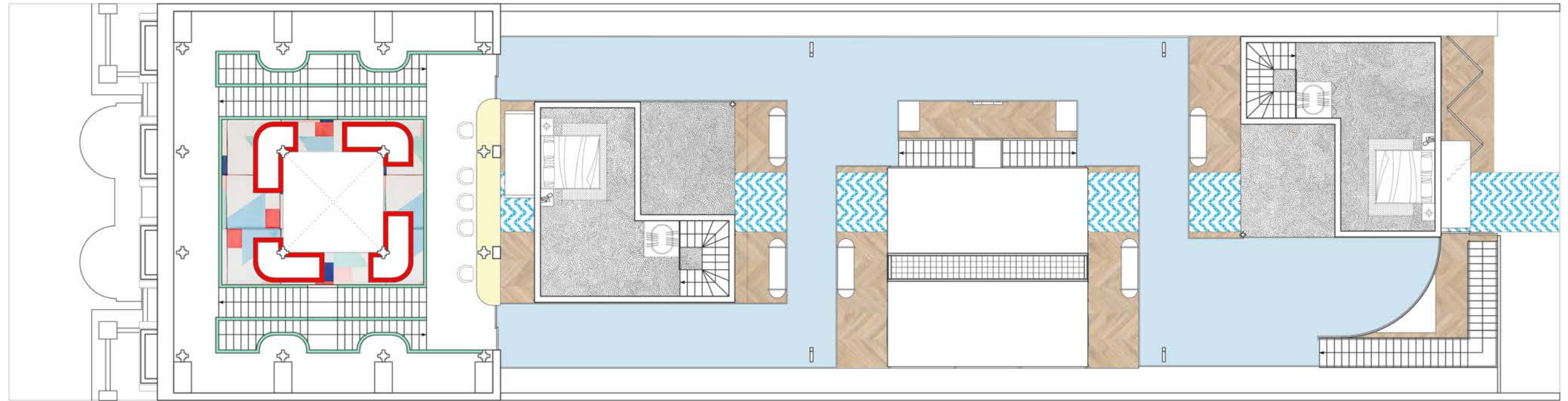
1:150@A3 Plan Level 4
