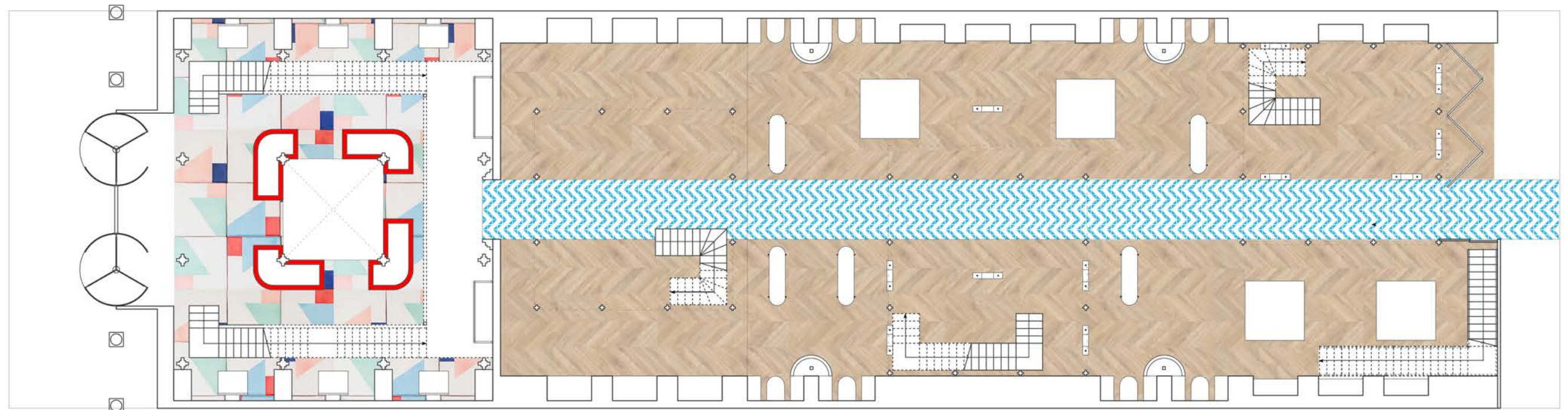
1:150@A3 Plan Ground Floor
