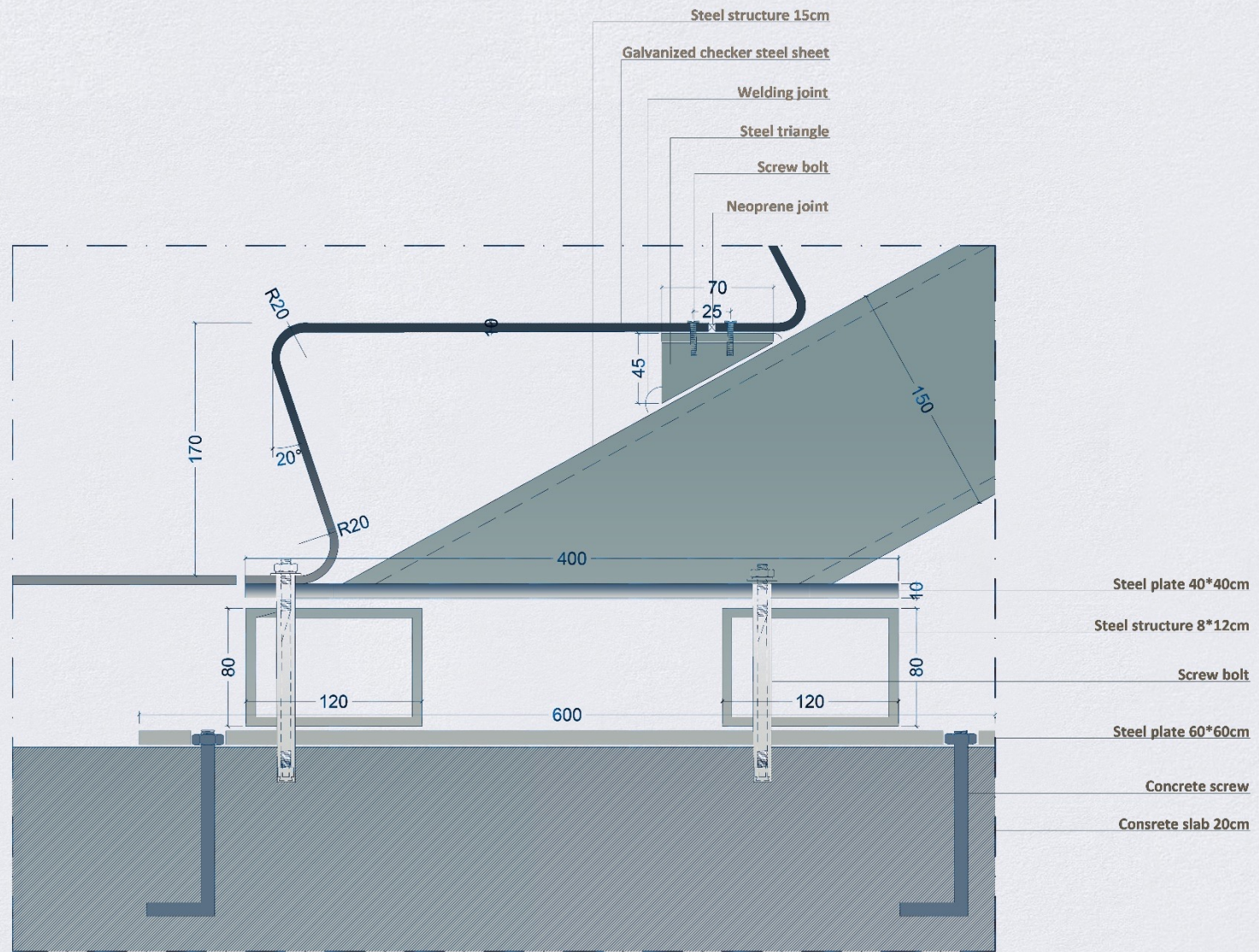
DETAIL 1 SCALE 1/1
