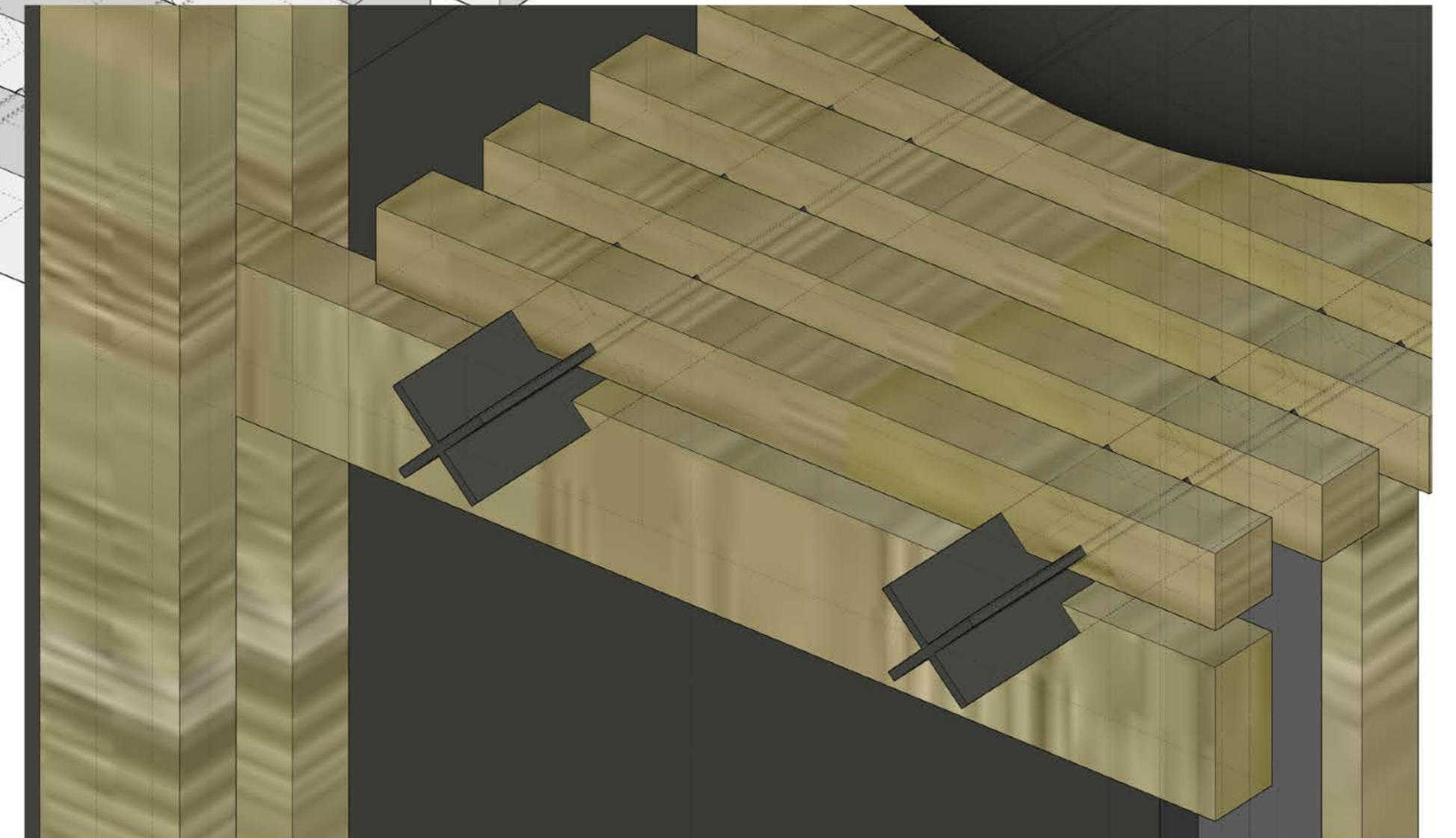
Self locking steel plate section passing through wood
