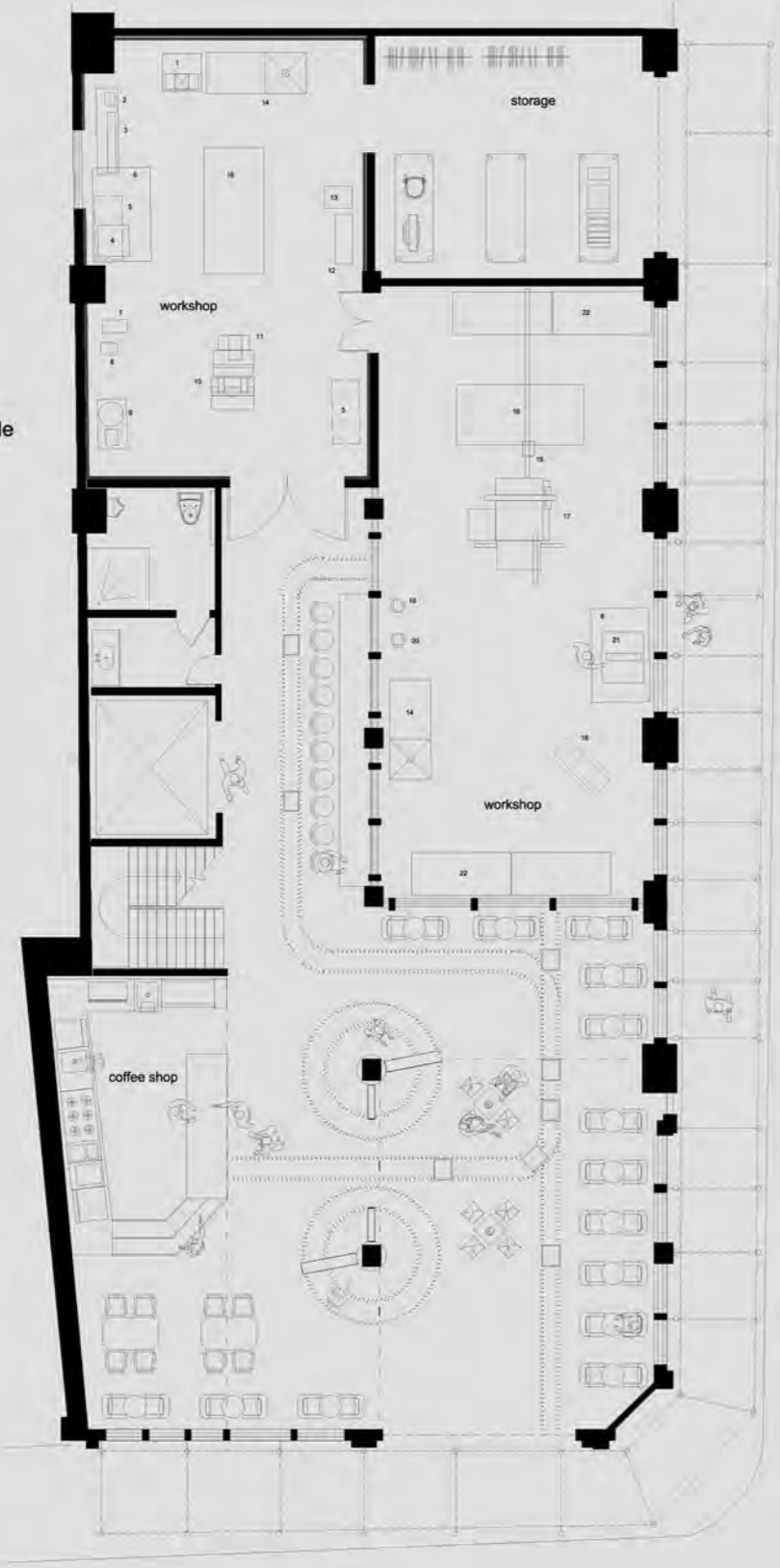
G1 PLAN 1:100
